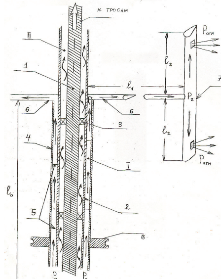
Figure 3 - Basic construction diagram of the turbine type H - Rotor
