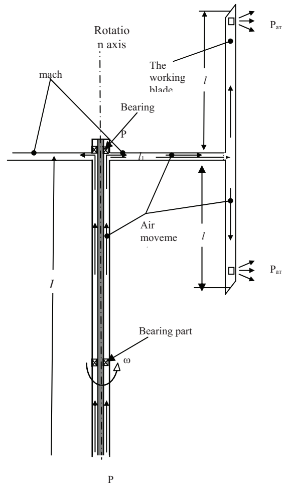
Figure 2 - Natural ventilation of air, as the result of working in centrifugal forces
