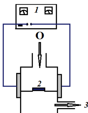
Figure 3 – Schematic representation of the installation for annealing: 1 – generator of ultra high frequency, 2 – sample, 3 – gas evacuation system
