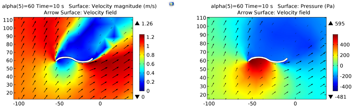
Figure 9 – Blade’s attack angle 60°
