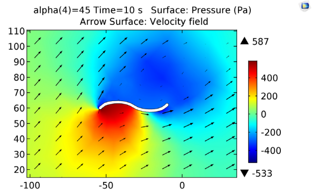
Figure 8 – Blade’s attack angle 45°
