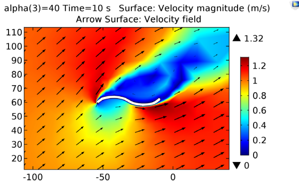
Figure 7 – Blade’s attack angle 40°
