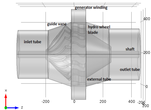
Figure 2 – Internal construction of the hydro turbine
