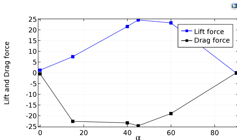
Figure 11 – Lift and drag force at last time
