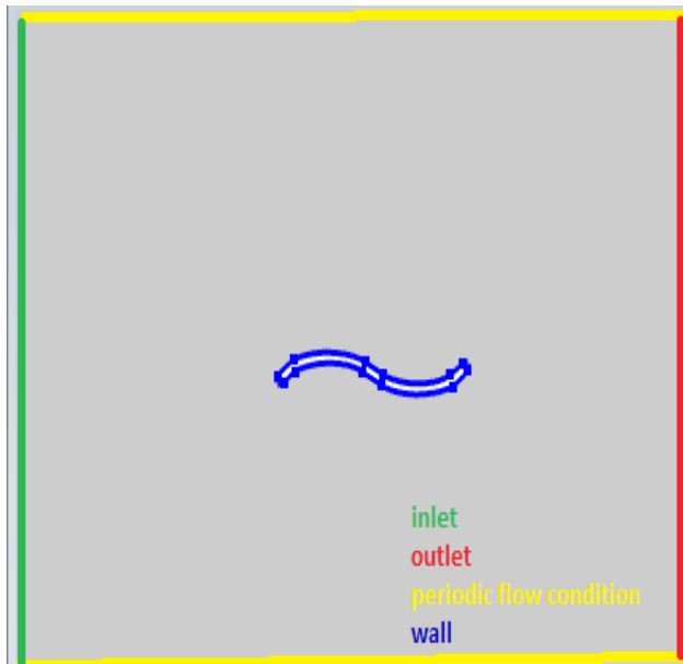
Figure 4 – Boundary conditions
