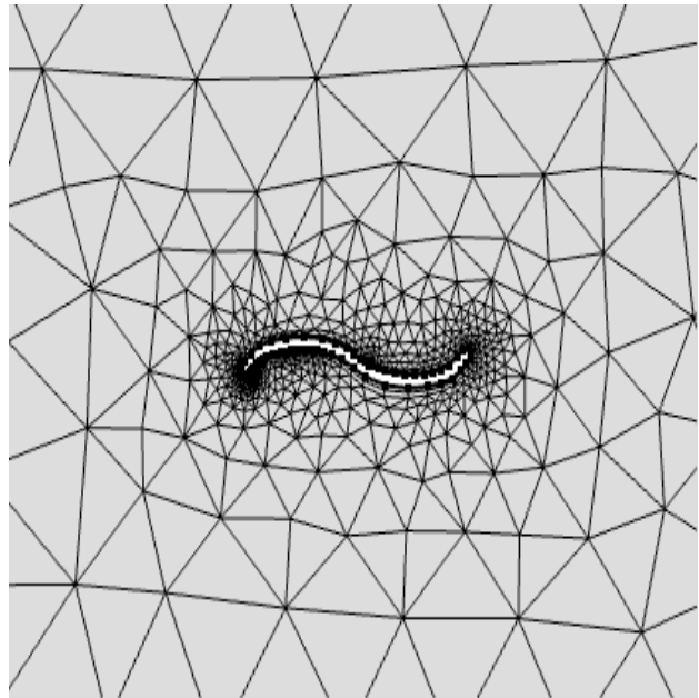
Figure 5 – Mesh allocation
