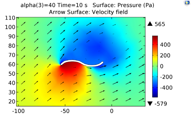
Figure 7 – Blade’s attack angle 40°
